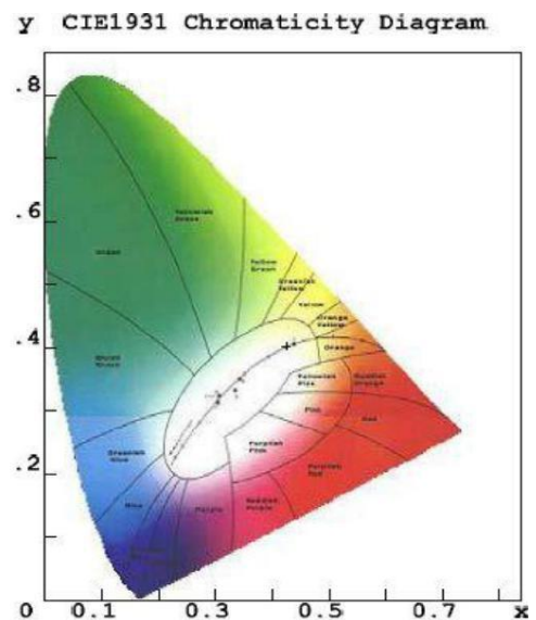
Chromaticity plot
